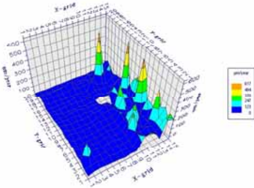
3-D Plot of corrosion rate
